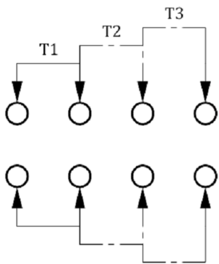
SCHEMATIC (NON-SHORTING)
